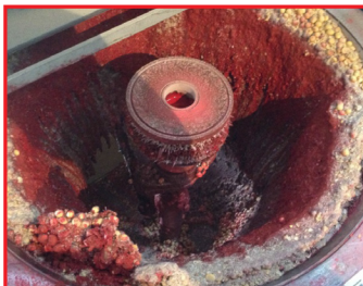
EXAMPLE OF A POORLY MAINTAINED BASKET ATOMIZER
